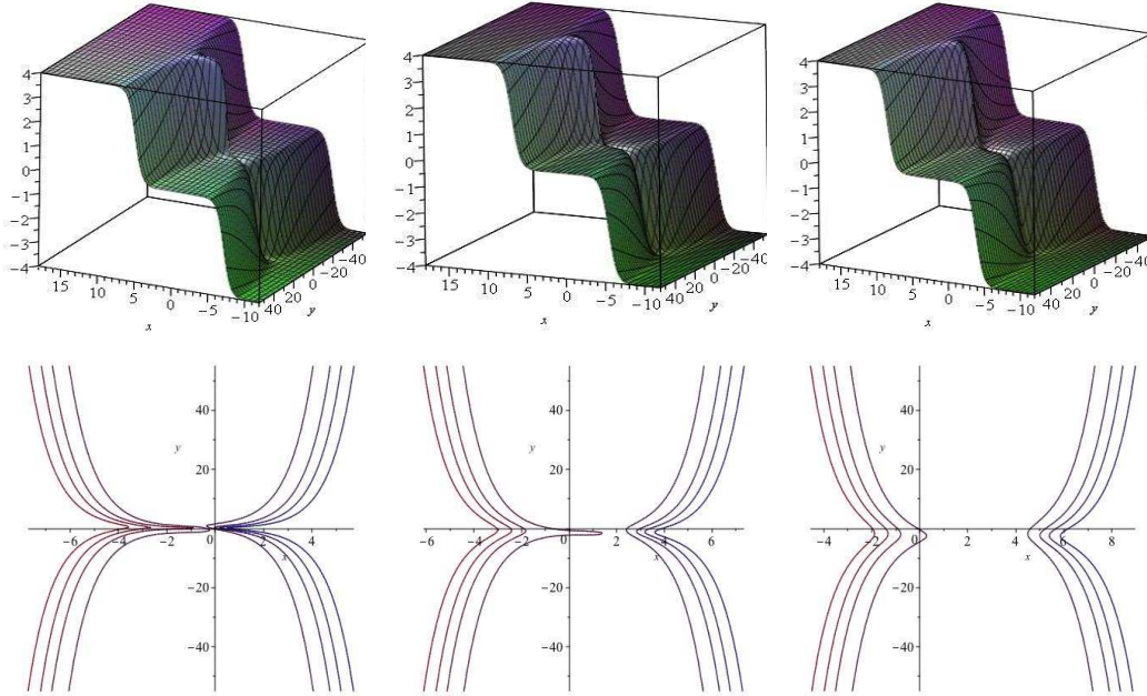
Figure 1: Solution of (2.6) for t = 0 , t = 0.1 and t = 0.2 . Top: 3d plots. Bottom: Contour plots.
