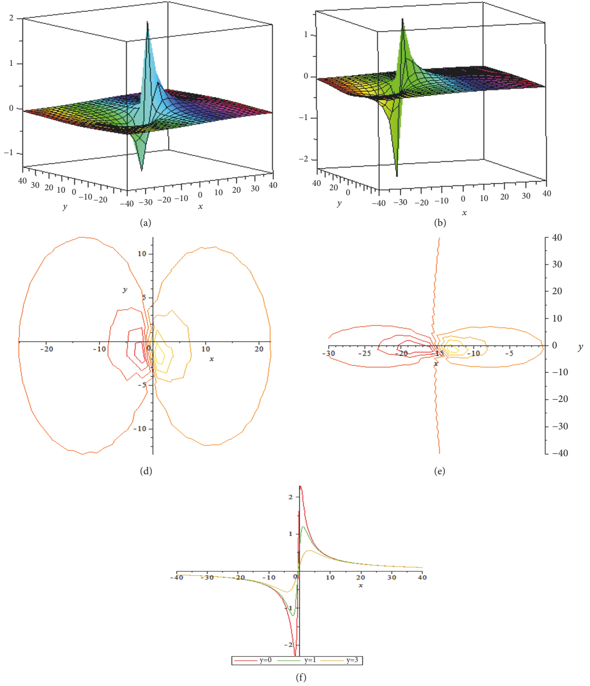
FIGURE 1: Proportion sight of the solution equation (8) with (6) and (5). For arbitrary constant values, \alpha_2 = \alpha_1 = 1, \alpha_7 = -1, \alpha_6 = 1, \alpha_{10} = 0, \alpha_{11} = 1 , and \alpha_8 = 5 . (a-b) 3D plots for t = 0 , and 3, respectively. (d-e) Consistent contour plot of (a), (b). 2D plot present in (f) for various values of y .
