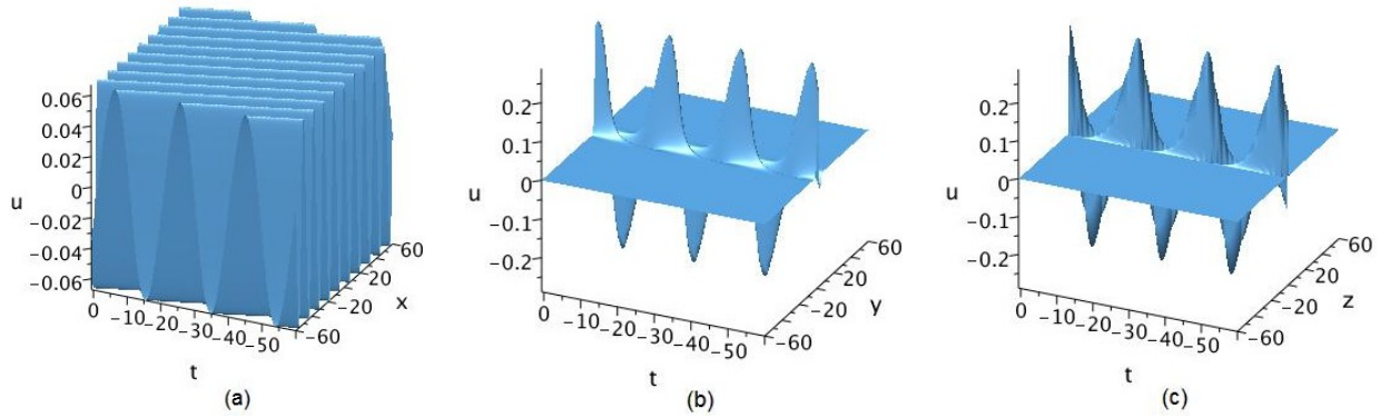
Fig. 2 – Periodic solitary wave solution (12): a) y = z = 0 ; b) x = z = 0 ; c) x = y = 0 .
