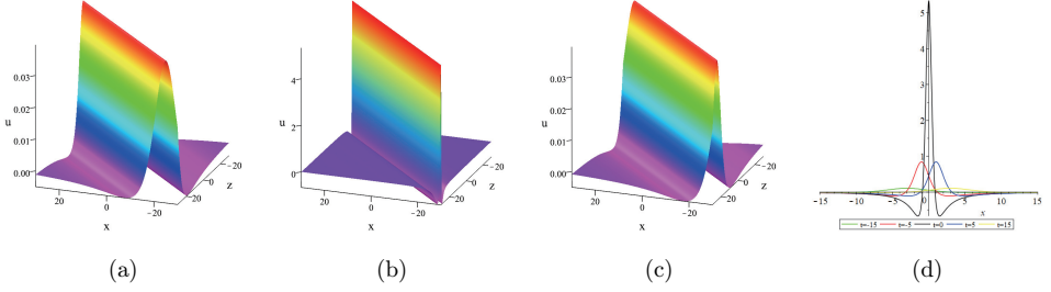
Fig. 7. (Color online) The time evolution of the one-line lump solution from (40) and (9) in the (x, z) -plane.
