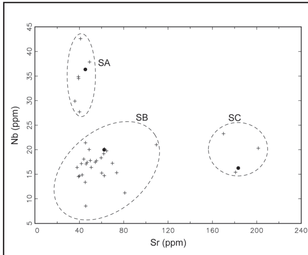
Fig. 3. Simple plot of strontium (Sr) versus Niobium (Nb) shows clear distinction between the major SA, SB, and SC subsources at Monte Arci.
