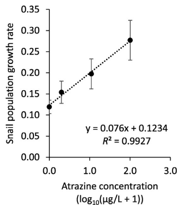
Fig. 1 The population growth rate of snails in outdoor mesocosms containing 0, 1, 10, 100 µg/L of atrazine in the Syngenta-funded study by Baxter et al. (2011). Growth rates are calculated for the exponential phase until a carrying capacity or decline in growth occurred. The 30 µg/L treatment was excluded because it did not show the same spatial blocking patterns in dissolved oxygen as the other treatments (see Rohr et al., 2012).
